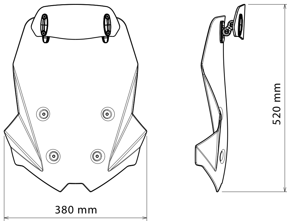
TOURING SCREEN WITH VISOR AT HIGHER POSITION
