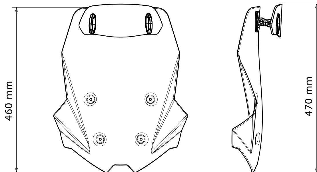
TOURING SCREEN WITH VISOR AT LOWER POSITION
